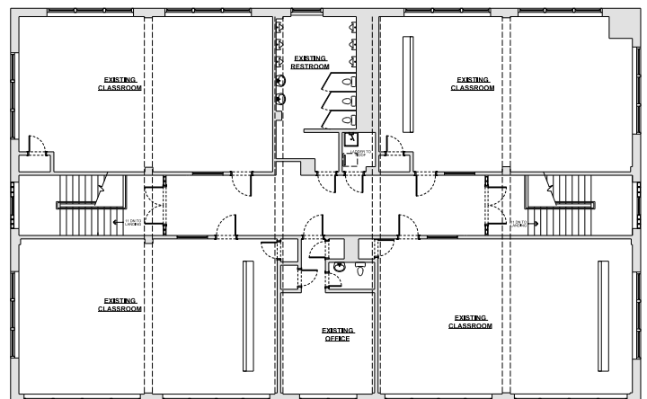
EXISTING SECOND FLOOR PLAN
