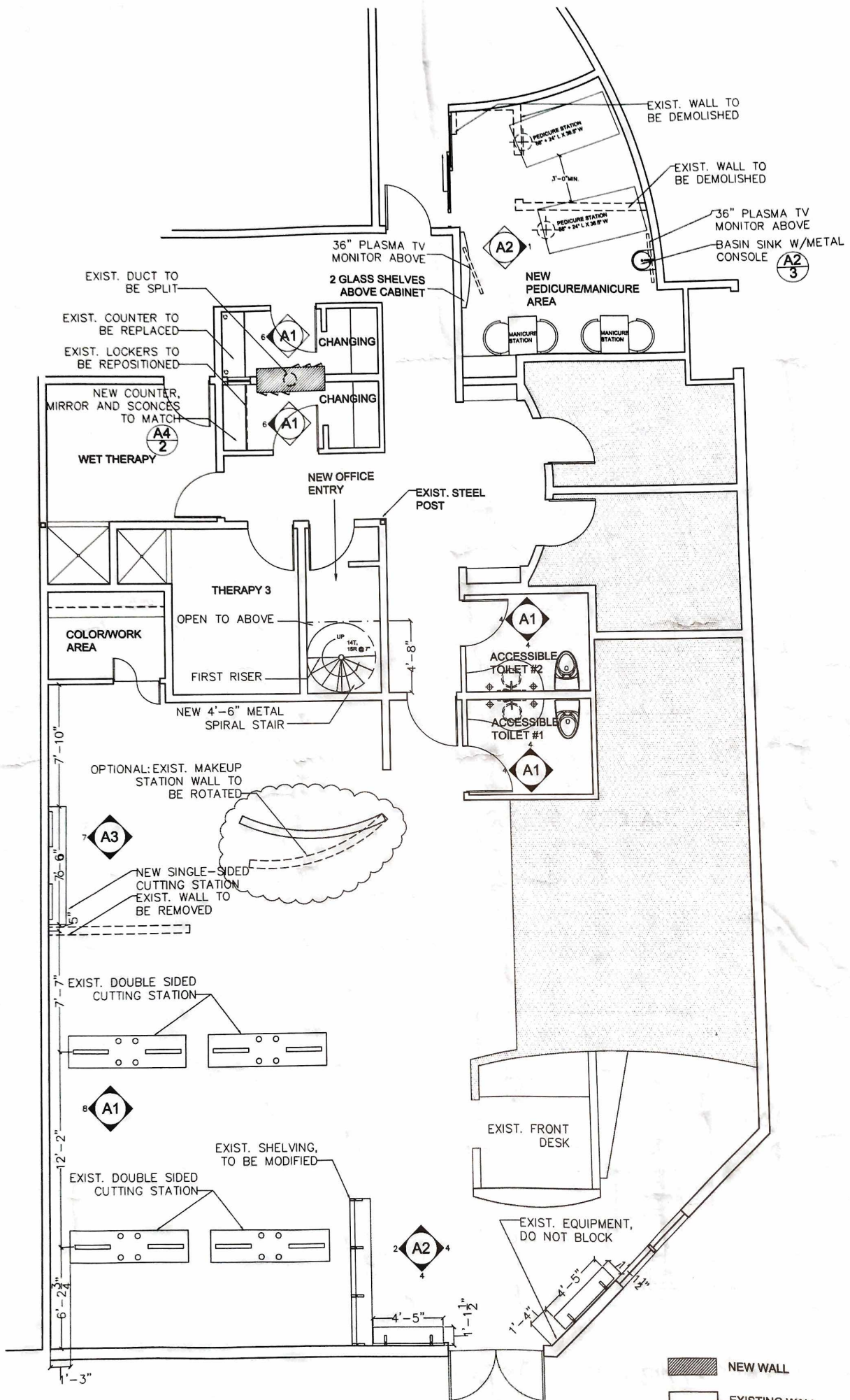
1 FLOOR PLAN SCALE: 1/4" = 1'-0"
