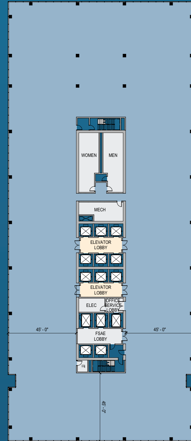
TYPICAL OFFICE | LEVEL 14-26
